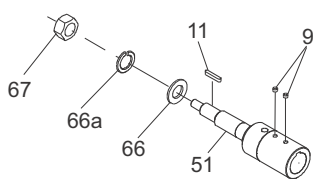
Stub shaft
